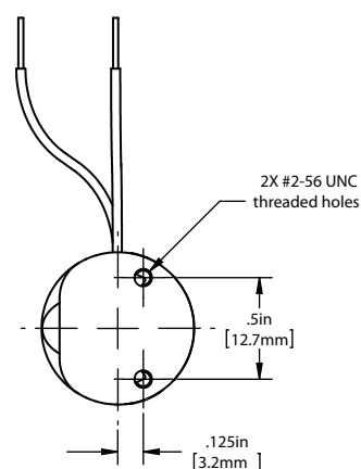
075P2NO 2-way Normally Open
