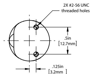
075P2NC 2-way Normally Closed
